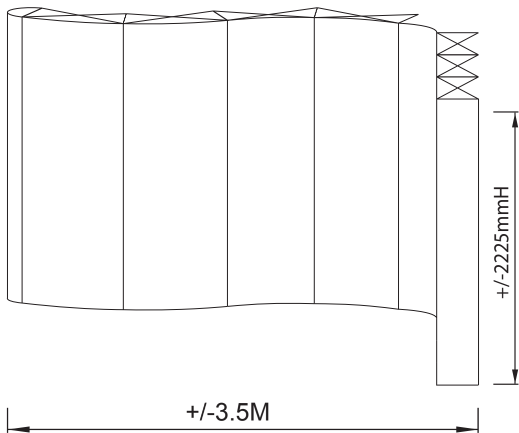
Front View - Stand Size
