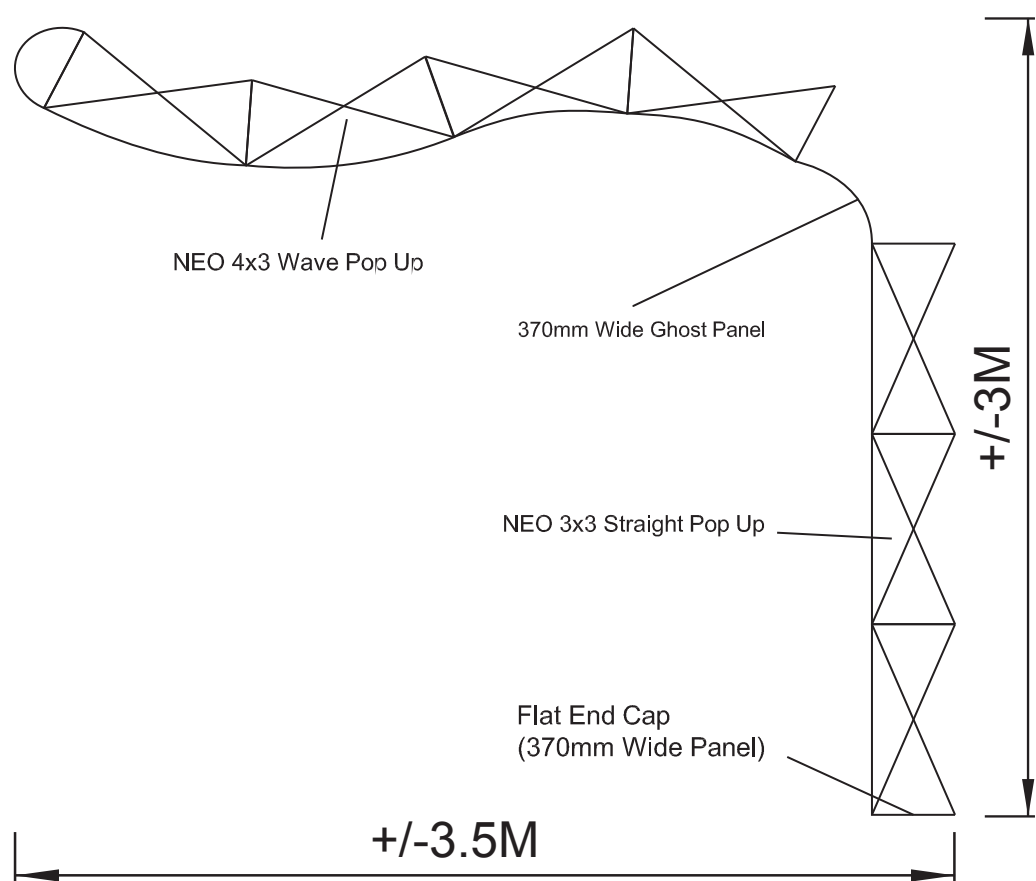
Top View - Stand Size
