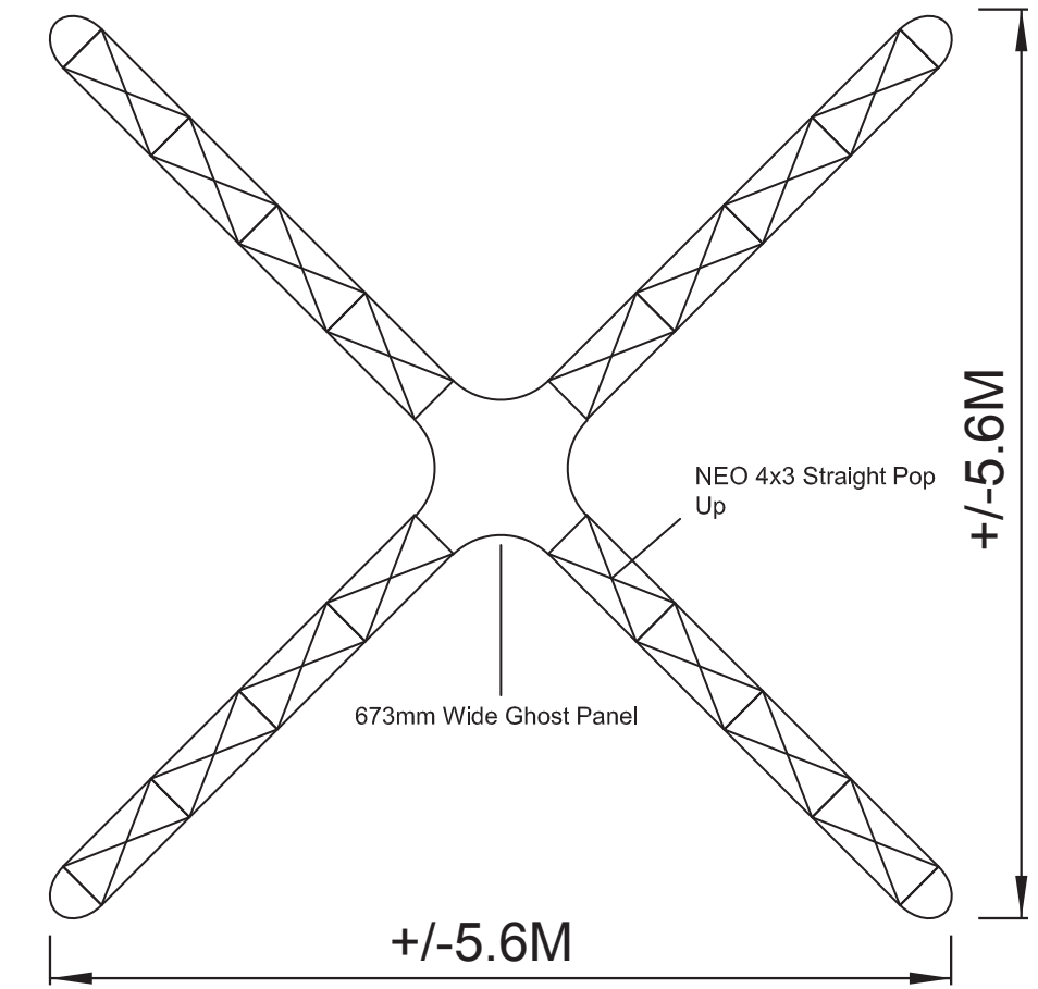
Top View - Stand Size
