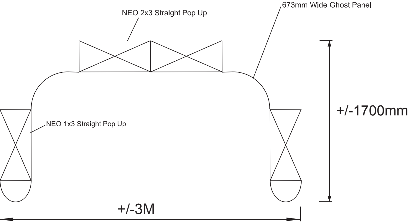
Top View - Stand Size
