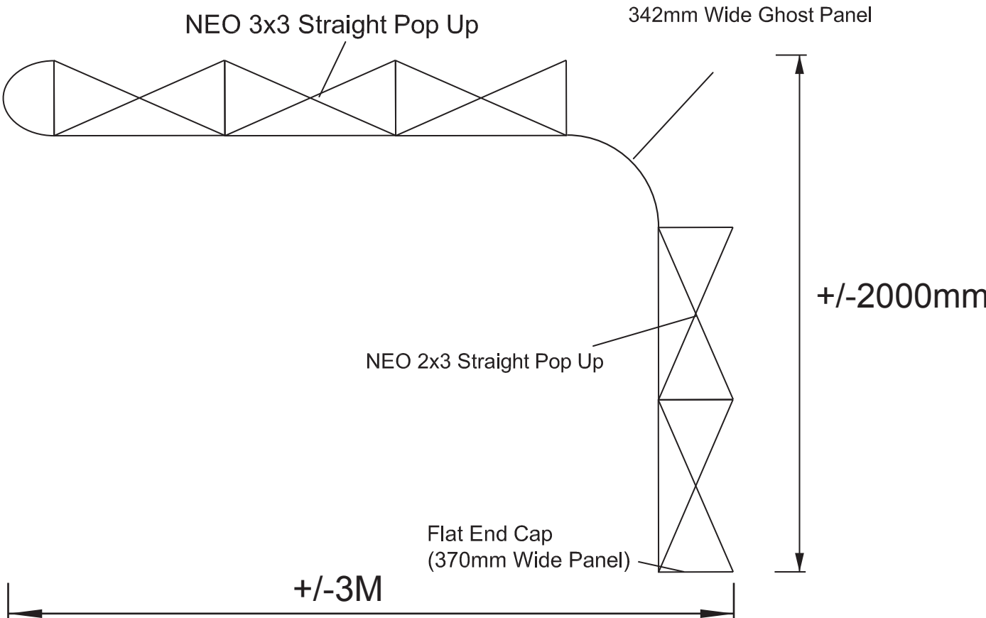
Top View - Stand Size
