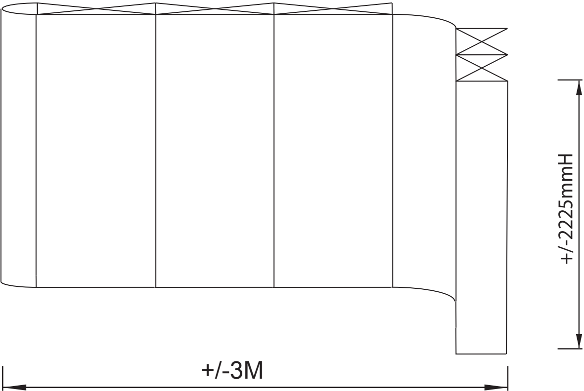
Top View - Stand Size
