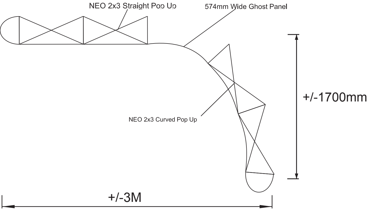
Top View - Stand Size
